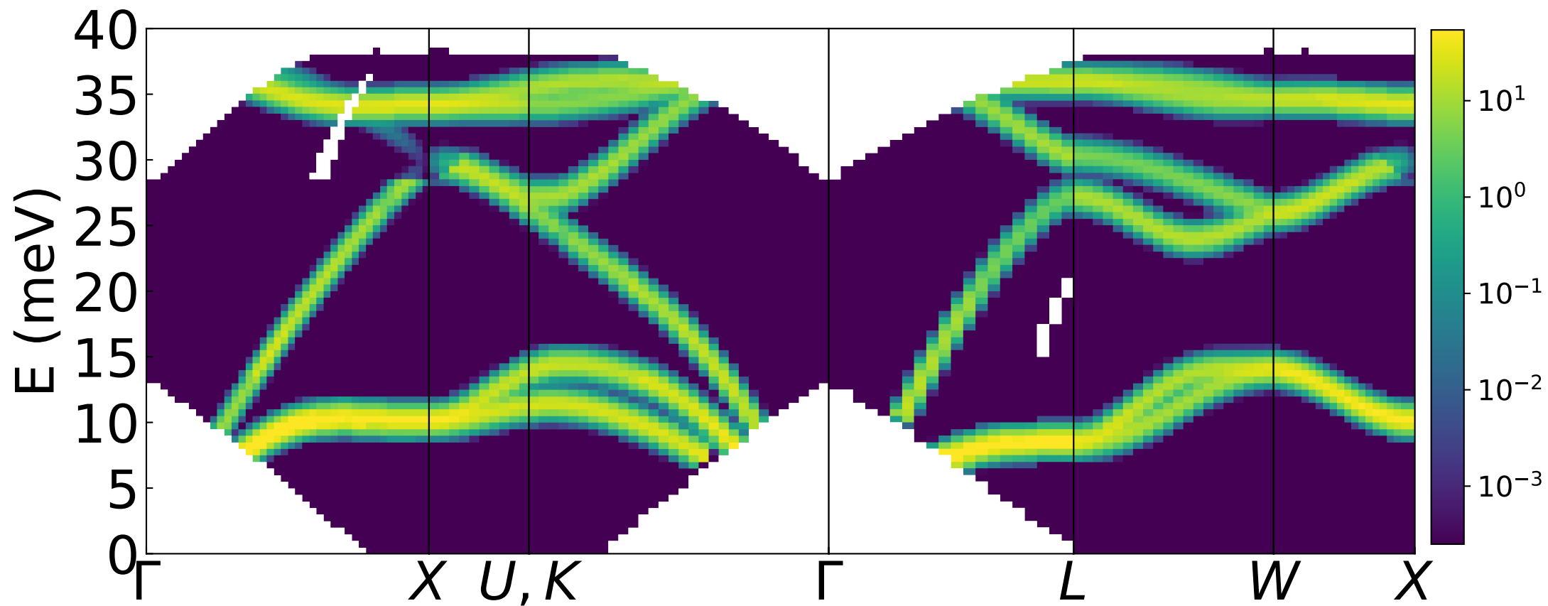
Folded simulated data along path in BZ [1 3 1]
