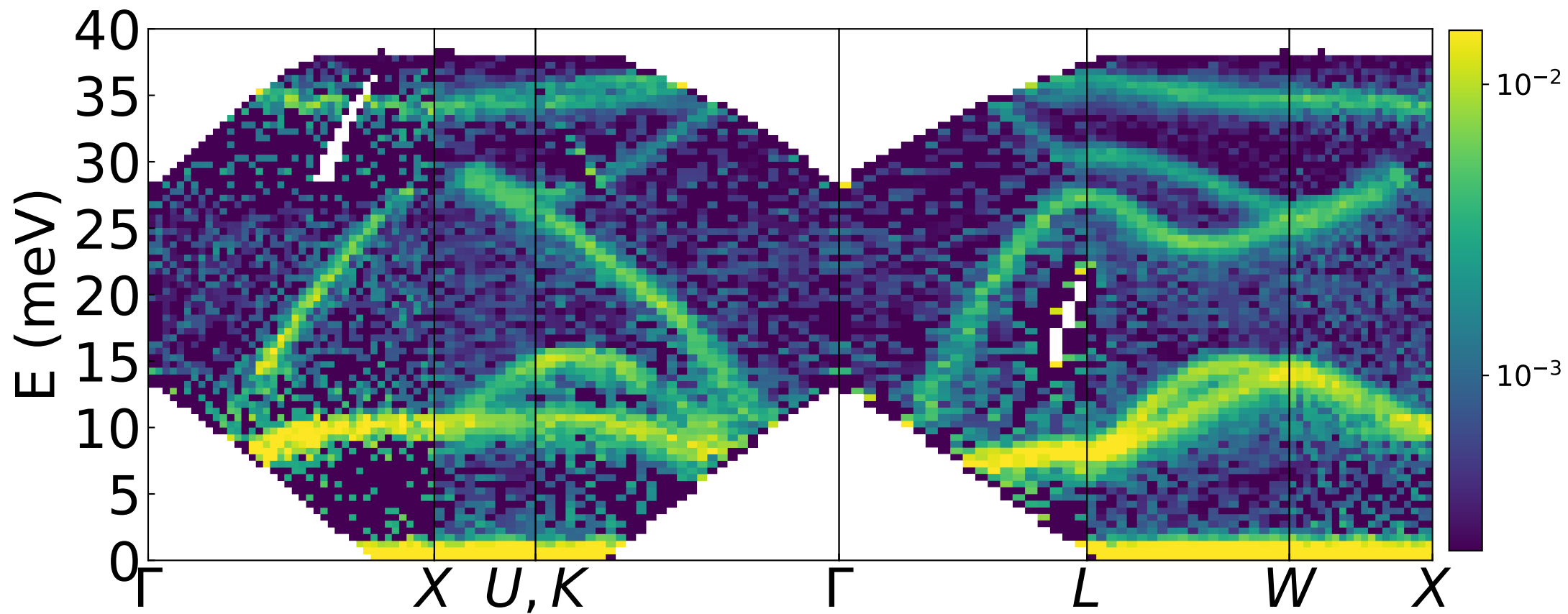
Folded experimental data along path in BZ [1 3 1]
